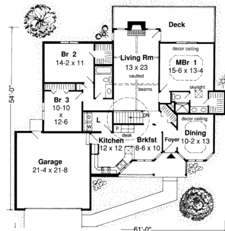
Slab/Crawl Space Option
